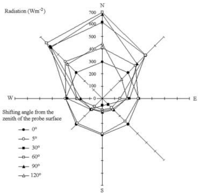
Fig. 2. Spatial distribution of 450–950 nm radiation on Strandline Glacier, 17 January 2003, 1200 h. Sun 35^{\circ} above the horizon, albedo 0.87.
