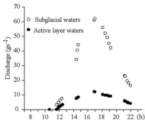
Fig. 9. Discharge of 4 January 2003. There is no runoff early in the morning, as water saturates the porosity. Between 1000 and 1200 h, water starts to flow. The flow rises far more quickly in the subglacial waters. Both peaks are at 1702 h, about 5 hours after maximum radiation.
