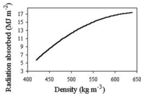
Fig. 3. Correlation between density and 450–950 nm radiation absorbed during the 24 hours (average) in snows having a radius of about 3 mm, and \alpha = 68\text{--}70\% . Surveys of 2–17 January 2003.
