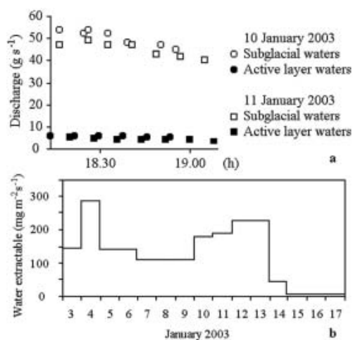
Fig. 10. (a) Comparison between the exhaustion of the discharge during two consecutive days. (b) Water extractable by gravity from lysimeter A. The 10–11 January discharge decreases, whereas extractable water rises. On the 14th, water was extracted at the lysimeter, but discharge was nil at the collecting points.
