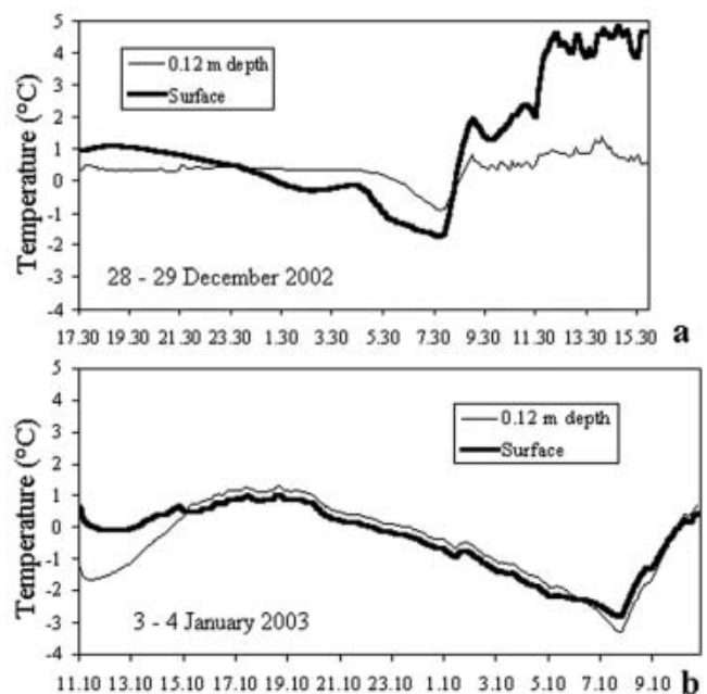
Fig. 6. Temperature measured every 2 min during good (a) and bad weather (b) on the surface and at 0.12 m depth. The probes are sheltered from direct sunlight. They are affected, however, by radiation diffused sideways into the ice and by radiation coming from the screen protecting them. If it is at melting point, the probe records a temperature ranging between +0.48^\circ\text{C} and +0.24^\circ\text{C} depending on radiation conditions.
