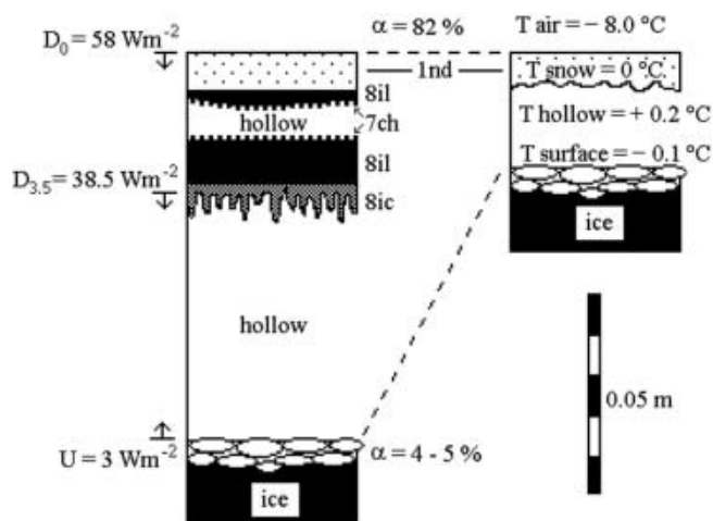
Fig. 15. Sections of M. Joyce Glacier flat surface. Lefthand side shows two hollows: an expanded one below, and an upper one still developing. On the righthand side there is only one hollow, in the initial phase of development. D: downward flux. ICSSG abbreviations (Colbeck and others, 1990).
