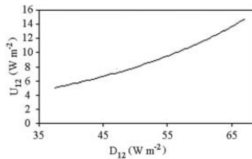
Fig. 5. D_{12} vs U_{12} . Average of period 2–17 January 2003.
