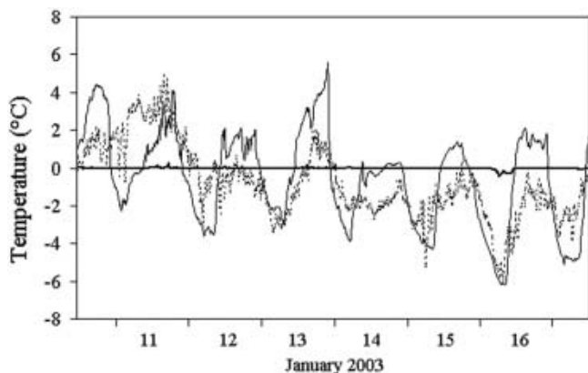
Fig. 7. Temperature trend at Eneide (air, dashed line) and at the Strandline Glacier surface (thin line) and 0.12 m depth (thick line). Highs and lows are more pronounced on the Strandline (slope with northerly exposure) than at Eneide (flat surface). Therefore the Strandline melting does not depend on a particular microclimate. Hence, it can be assumed that similar processes also take place on the other glaciers of Terra Nova Bay.
