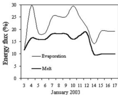
Fig. 13. Percentage of absorbed energy due to melt (thick line) and evaporation (thin line) at the lysimeters, assuming average irradiance measured at Eneide to be 100%.
