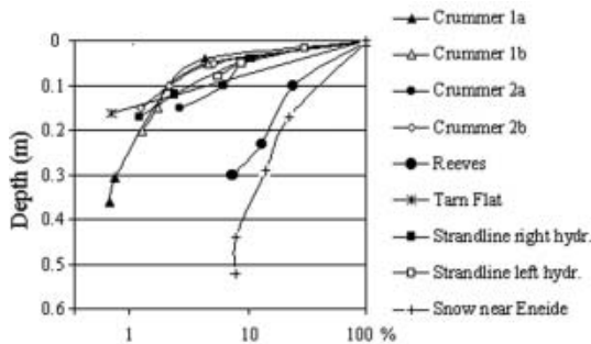
Fig. 12. Percentages of absorption of downward flux recorded during 2000–01 and 2002–03. The measurement method used is the same as for Strandline Glacier. The trend is very similar in all ablation zones of the alpine local glaciers, snow-clad (Strandline, Crummer 1a, 1b, 2b) or with clean ice (Crummer 2a, Tarn Flat, Strandline). Reeves Glacier (an outlet glacier) blue ice and the seasonal snowpack (Eneide) are more transparent.
