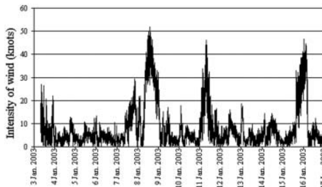
Fig. 14. Wind ( 1\ \text{knot} = 1.85\ \text{km h}^{-1} ) at the weather station Eneide. The katabatic winds alternate with very weak winds.
