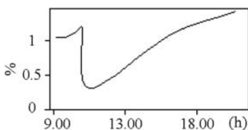
Fig. 4. Per cent of irradiance at 0.12 m depth. Average of period 2–17 January 2003.
