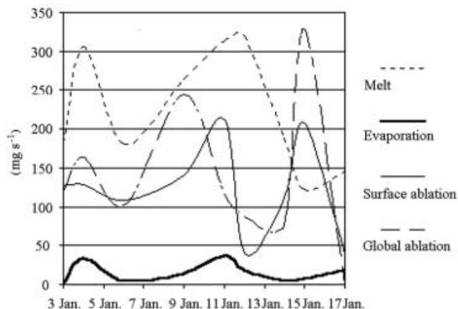
Fig. 8. Daily values of melt, evaporation, superficial and total ablation recorded in 2003. Melting and evaporation refer to the lysimeters, surface ablation to the ablatometric stake. Global ablation is the balance of density variations of the snow and surface ablation.
