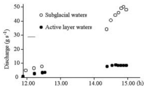
Fig. 11. Effects of clouding on the flow, at 1447 h, 5 January. The subglacial flow decreased a few minutes after the sun shading, while the water flow in the active layer remained constant. This shows that the medium lag between the input event and the output response of the subglacial water lasts a few minutes (short travel).
