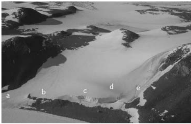
Fig. 1. Strandline Glacier. a: transition between a ramp and a dome front; b and d: dome fronts; c: cliff; e: ramp front.
