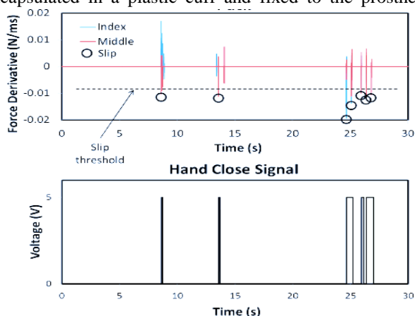
FIGURE 10. Grasping trial performed in [136]. Negative peaks in the derivative signal produced spikes triggering the prosthesis closure.
