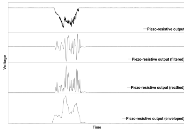
FIGURE 6. Signal elaboration according to [100].
