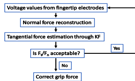
FIGURE 7. Flow chart of the algorithm developed in [104] (readapted). Normal force was reconstructed from the fingertip electrodes output. Tangential force was estimated on the electrodes output through the KF. Force ratio determined whether to correct the grip force or not.
