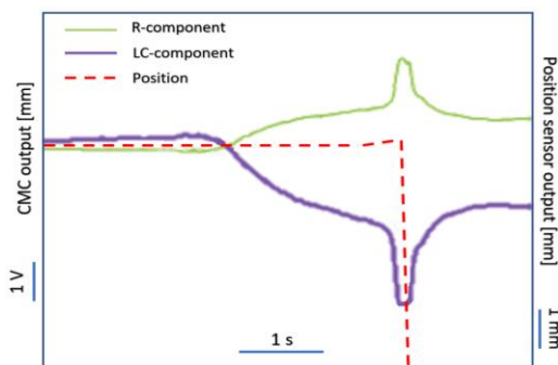
FIGURE 9. CMC sensor output for a typical trial. Both R-component and LC-component showed sudden variation when slip occurred. Readapted from [128].
