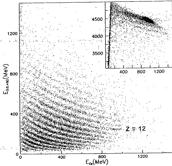
Fig. 6. Scatter plot of the IC+Si energy loss vs the CsI residual energy. In the insert the Z values around Xe are shown.
