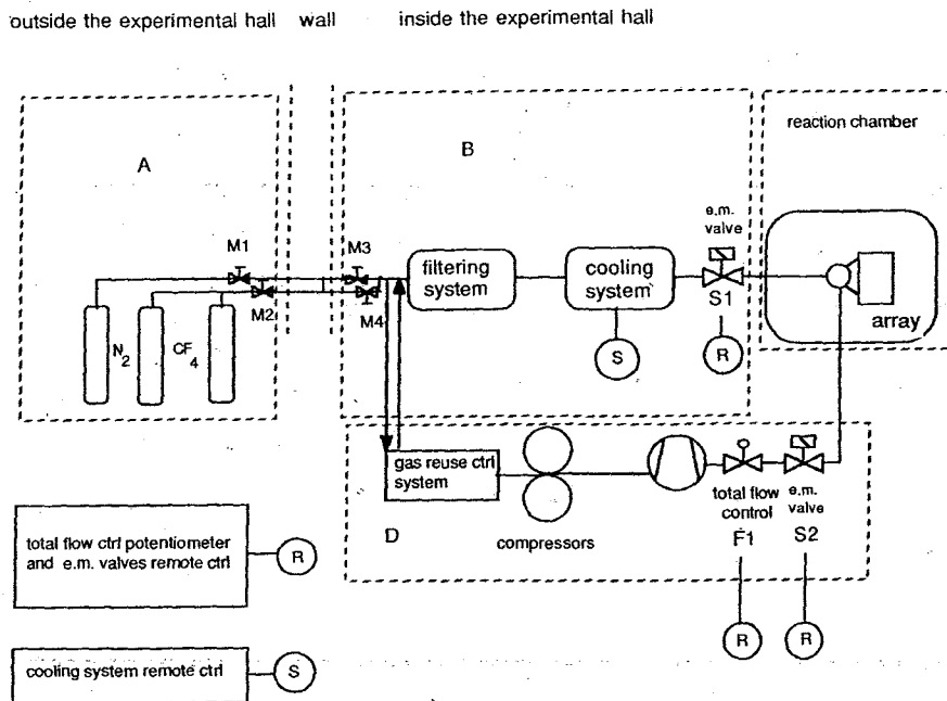
Fig. 4. Overview diagram of the gas system.
