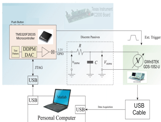
FIGURE 12. Experimental test setup.
