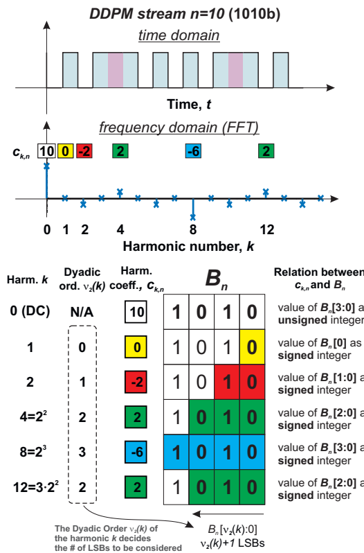
FIGURE 2. Illustration of the relation between the harmonic spectral coefficients c_{k,n} and the binary representation B_n of the digital input code n , as presented in [8], for the digital input n = 10 (i.e. B_n = (1, 0, 1, 0) ).
