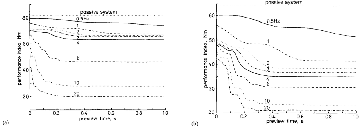
Fig. 28. Resulting cost function values (referred to as performance index) as functions of preview time for controller calibrations targeting: (a) handling improvement; and (b) ride comfort improvement, for different suspension actuator cut-off frequencies, on a random road profile at constant speed (10 m/s). Reproduced with permission from Prokop and Sharp (1995).
