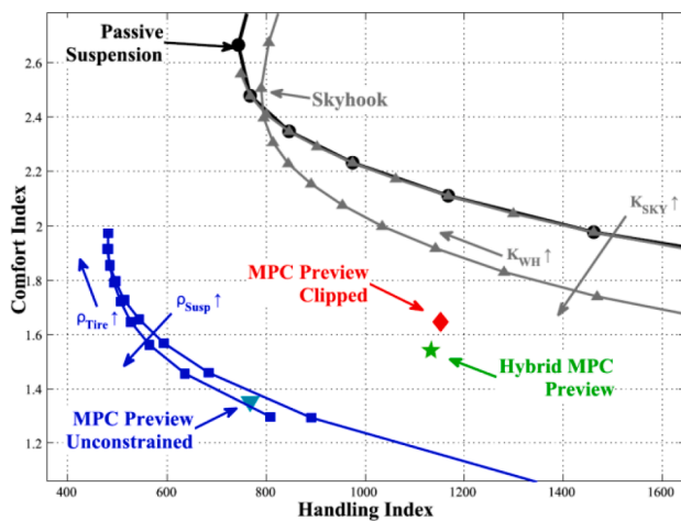
Fig. 19. Conflict diagram for the vehicle with the passive set-up (circles), with a skyhook controller (triangles), and with a preview-augmented unconstrained MPC (squares), driven over a sinusoidal bump. For one setting of the cost function weights, the plot also includes the comparison among the following iMPCs: i) an unconstrained MPC with preview ('MPC Preview Unconstrained'); ii) a clipped MPC with preview ('MPC Preview Clipped'); and iii) the proposed hybrid MPC approach with preview ('Hybrid MPC Preview'). \rho_{Tire} = \rho_2 and \rho_{Susp} = \rho_3 are the tyre deflection and suspension stroke weights in (29); k_{SKY} is the skyhook gain; and k_{WH} is the wheel hop gain (see the original reference for more details). Reproduced with permission from De Bruyne et al. (2012).
