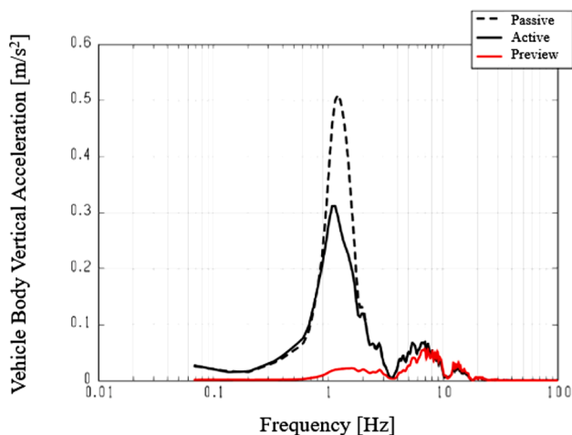
Fig. 6. Simulation results of vehicle body vertical acceleration frequency content on a ride comfort assessment road for: i) the passive set-up ('Passive'); ii) the vehicle with the active suspension controller with feedback contribution only ('Active'); and iii) the vehicle with the integrated preview strategy ('Preview'). Reproduced from Schindler (2009).
