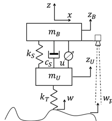
Fig. 9. Schematic of the quarter car model with active suspension actuator in parallel with the passive components.
