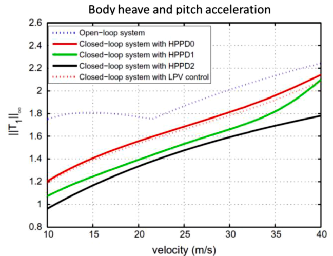
Fig. 17. H_\infty norm of the transfer function T_1 from the road input profile to the body vertical and pitch accelerations for the considered configurations, as a function of vehicle speed. Reproduced with permission from P. Li et al. (2014b).
