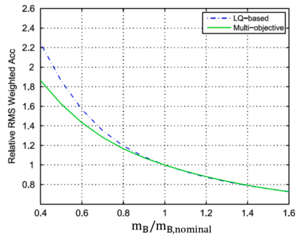
Fig. 16. Relative WRMS values of vertical body acceleration for the multi-objective and LQ-based controllers, as functions of the non-dimensional sprung mass value, for a realistic road input profile. Reproduced with permission from Akbari and Lohmann (2010).
