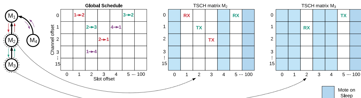
FIGURE 1. Example of a TSCH matrix defining the slotframe usage: global schedule (on the left) and local, trimmed-down copies (on the right).
