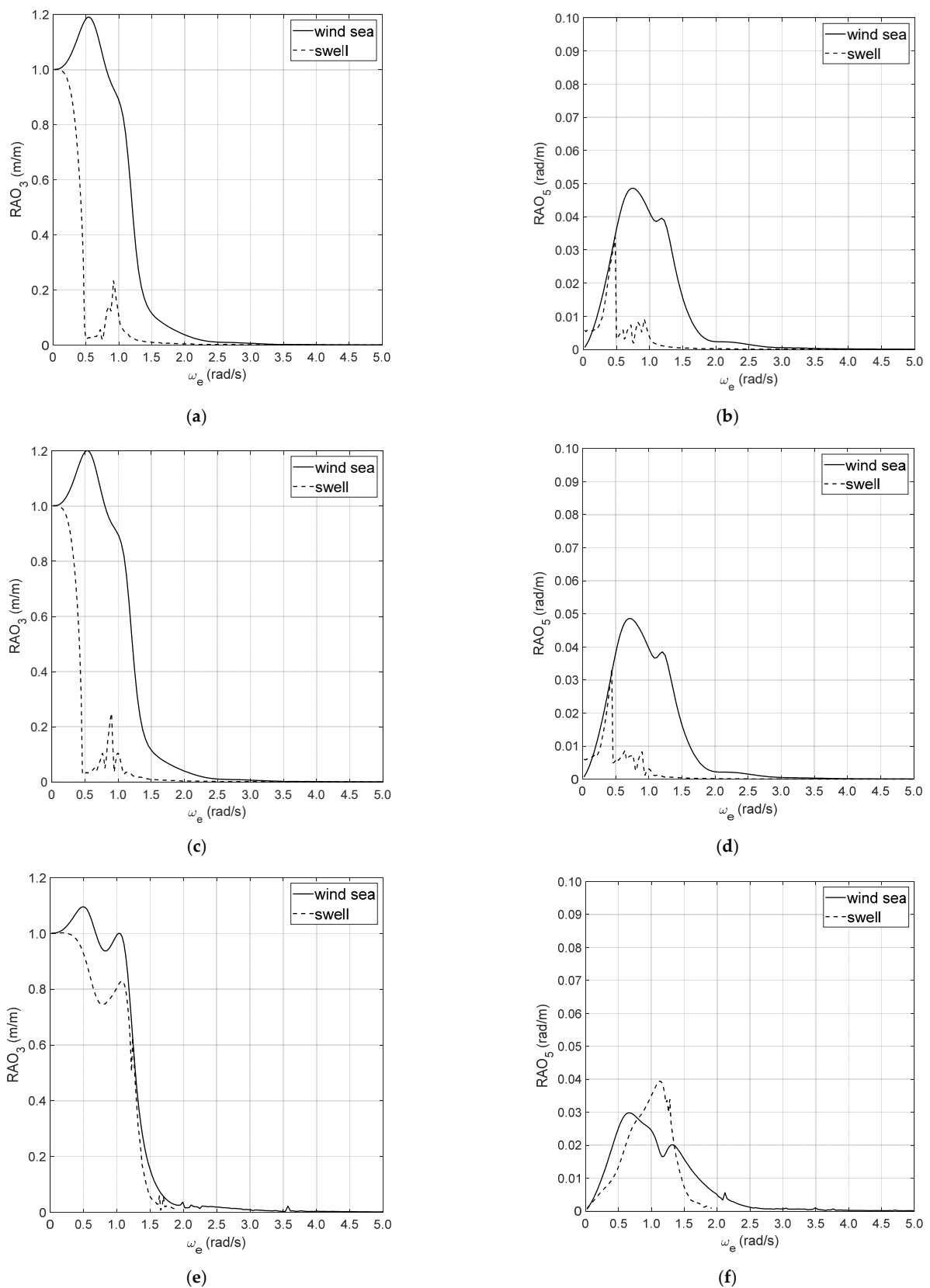
Figure 4. Heave and pitch RAOs (Response Amplitude Operator) in the encounter frequency-domain: (a) heave—7 January 2020; (b) pitch—7 January 2020; (c) heave—8 January 2020; (d) pitch—8 January 2020; (e) heave—14 February 2020; (f) pitch—14 February 2020.
