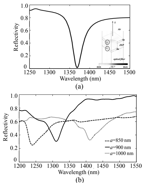
Fig. 6 Theoretical analysis of hybrid nanostructures realized on the fiber facet: (a) reflectance spectra of the analyzed nanostructure; (inset) 3D view of 1/4 of unit cell and electric field intensity distribution evaluated at the reflectance dip wavelength) and (b) reflectivity of hybrid structures characterized by different periods ( a=850 nm, 900 nm, and 1000 nm) [16].
