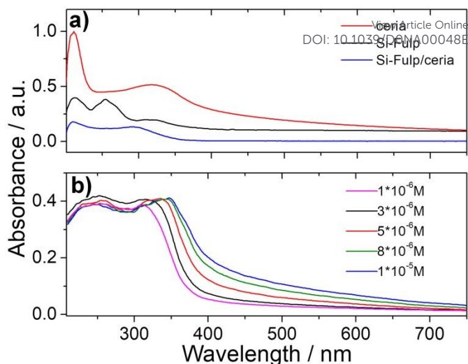
Fig. 7 a) UV-Vis spectroscopy of nanoceria, Si-Fulp and Si-Fulp/ceria in water solution. b) UV-Vis spectra of Si-Fulp/ceria in water at different concentrations.
