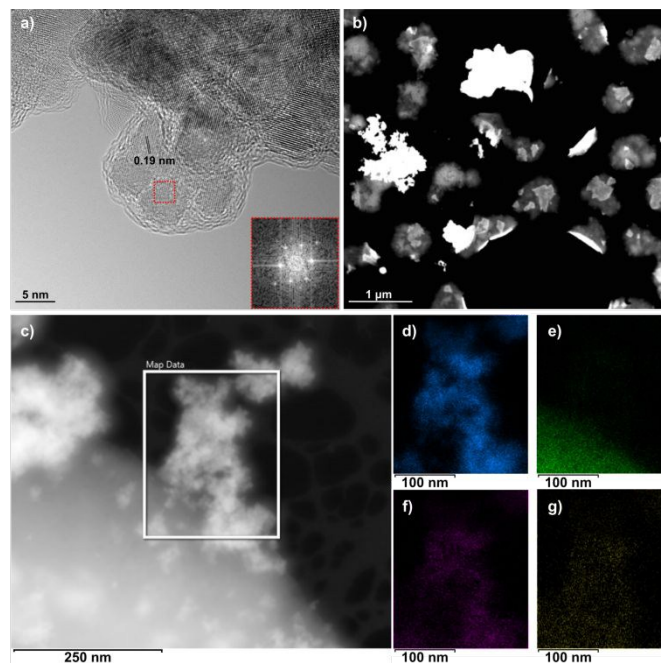
Fig. 4 a) HR-TEM and b) DF-STEM images of Si-Fulp/ceria. The inset in a) shows the FFT obtained on the nanoceria (red-boxed region) with a d -spacing of 0.19 nm. c) Transmission electron image of Si-Fulp/ceria. EDS elemental maps of d) Ce, e) C, f) O, g) Si obtained on the boxed region in c).
