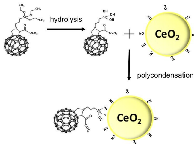
Fig. 1 Diagram of the nanoceria functionalization with Si-Fulp.
