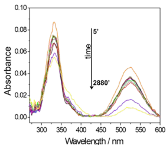
Fig. 8 UV-Vis spectroscopy of a Si-Fulp/ceria dispersed in DPPH water solution (0.078 mg mL -1 ) as a function of time (min.).
