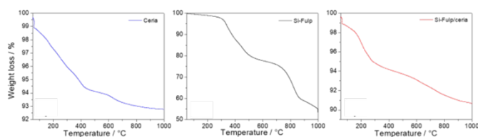
Fig. 6 TGA analysis of nanoceria (blue line), Si-Fulp (black line) and Si-Fulp/ceria (red line) in air at a heating rate of 10 °C
