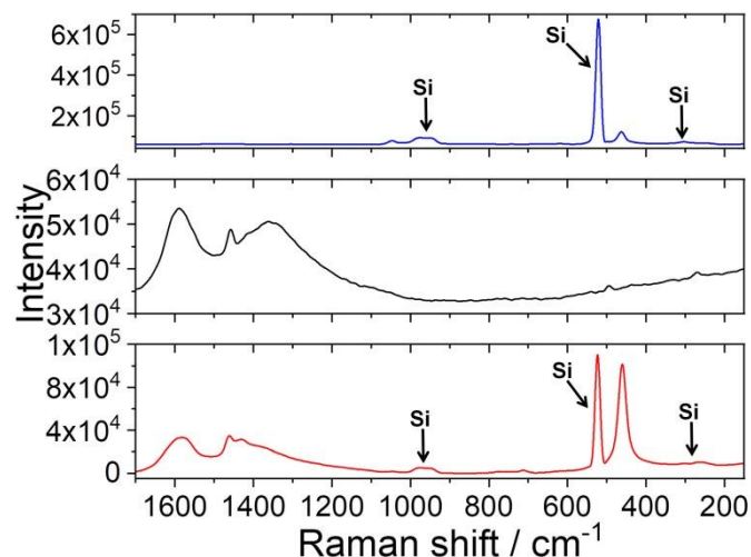
Fig. 2 Raman spectra in the 1700 – 150 cm -1 range of nanoceria (blue line), the pristine Si-Fulp (black line) and nanoceria functionalized with Si-Fulp (red line). The bands at 303, 523 and 965 cm -1 are due to the monocrystalline silicon substrate.
