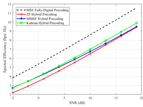
(c) Achievable rate in 10 paths scenario
