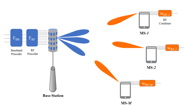
FIGURE 1. MmWave multi-user system model: BS hybrid analog/digital precoding and MS analog combining.
