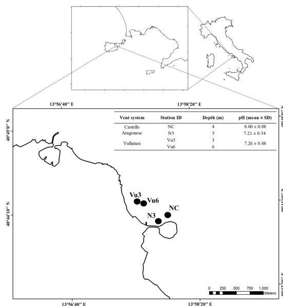
Fig. 1: Map of the study area (Ischia, Italy) showing the locations of stations (N3, Vu3, Vu6, and the control). The table reports on the right corner which of the vent systems the station belongs to, the station's identification code (ID), the depth, and the mean ± SD of pH measured.
