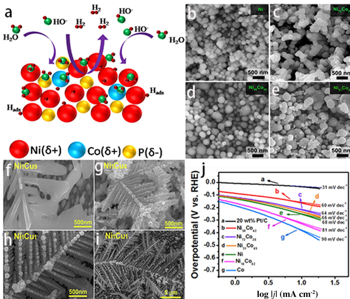
Fig. 16 a Schematic illustration of electrocatalytic HER on the surface of catalysts in alkaline media [248]. b–e SEM images of mesostructured \text{Ni}_{100-x}\text{Co}_x alloys prepared from different LLC compo-
