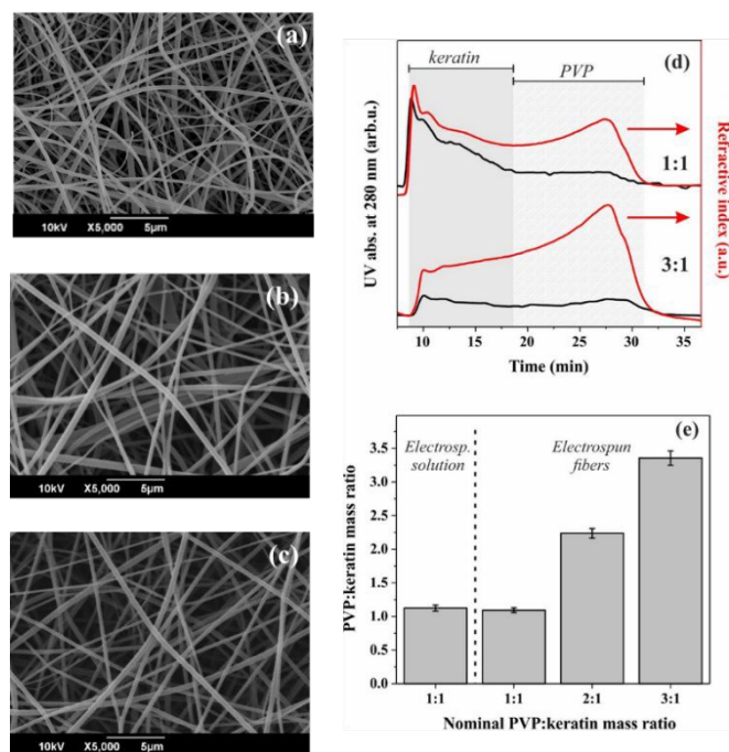
Figure 1 SEM images of PVP:keratin fibers electrospun from solutions at different mass ratios, (a) 3:1, (b) 2:1 and (c) 1:1; (d) Representative AF4 analyses for the 1:1 (above) and 3:1 (below) PVP:keratin fibers; the refractive index detector traces (red curves, right axis) provides peaks corresponding to the elution of both materials, but its comparison with UV absorption (black curves, left axis) allows the clearer identification of keratin. (e) The experimental values of the mass PVP/keratin mass ratio were obtained through appropriate calibration of the regions in the AF4 elugrams; the comparison between the composition of the solution used for electrospinning and the electrospun fibers (first two columns from the left) shows no significant deviation of the material composition from that of its feed. Further, the mass ratio between the two components of the fibers was always close to its theoretical value.
