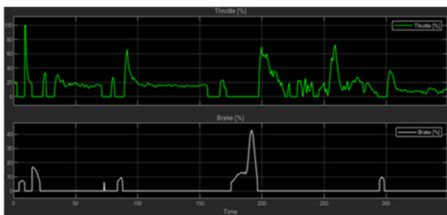
Fig. 12 Throttle and brake signals
