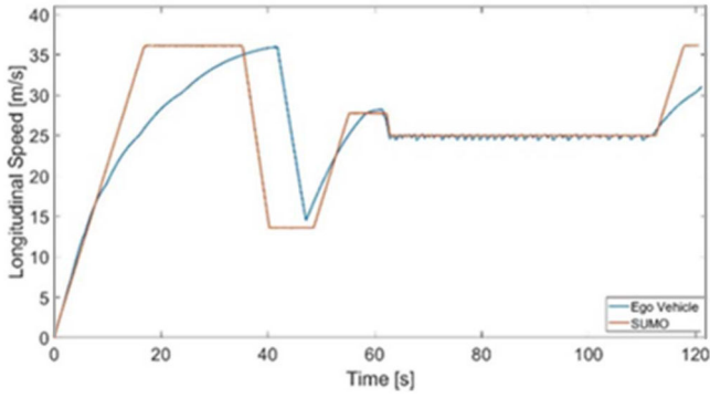
Fig. 6 Speed profile for the Ego-Vehicle in Test 1
