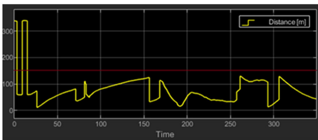
Fig. 11 Distance from leader and radar threshold
