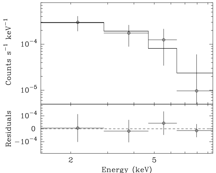
FIG. 2.— X-ray spectrum of 4U 0115+63 as observed by BeppoSAX MECS. The overlaid model is a power law with interstellar absorption (see text). Residuals are shown in the lower panel.
