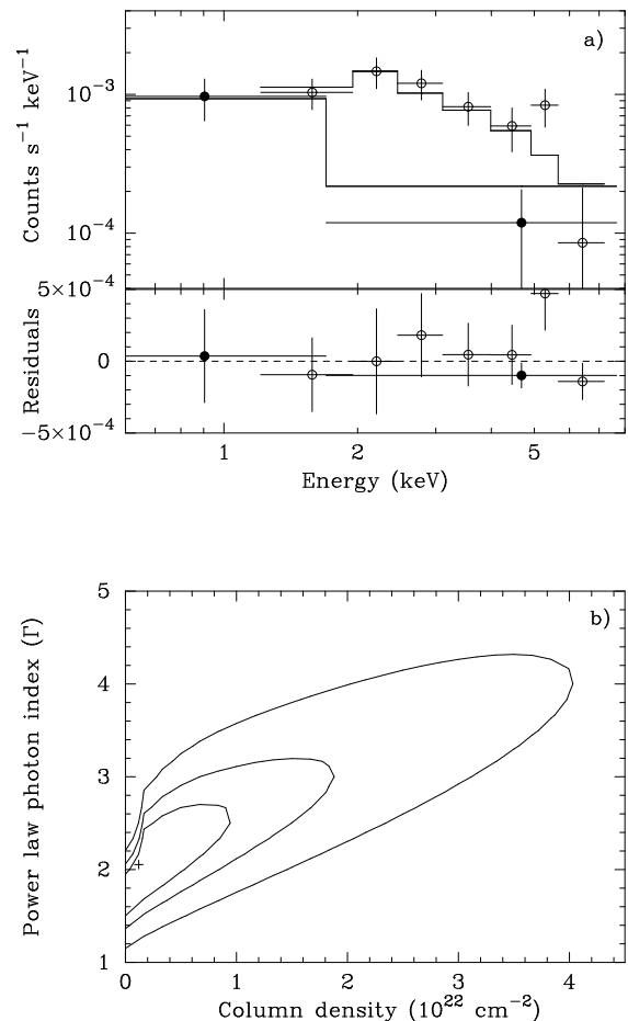
FIG. 1.— Panel a): X-ray spectrum of A 0538–66 as observed by BeppoSAX. Filled and open circles refers to LECS and MECS data, respectively. The overlaid model is a power law with interstellar absorption (see text). Residuals are shown in the lower panel. Panel b): contour plot of the power law photon index versus the column density. Contours are at a level of 1, 2 and 3 \sigma .
